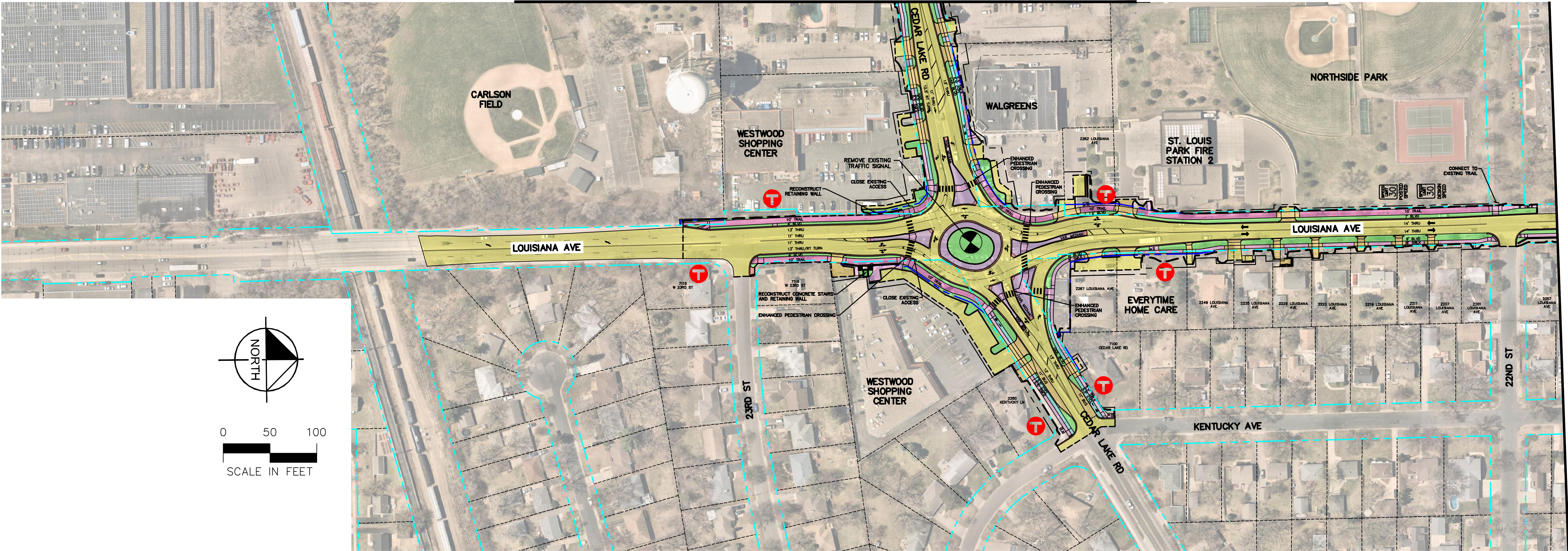
MATCH LINE SEE CEDAR LAKE ROAD LAYOUT
