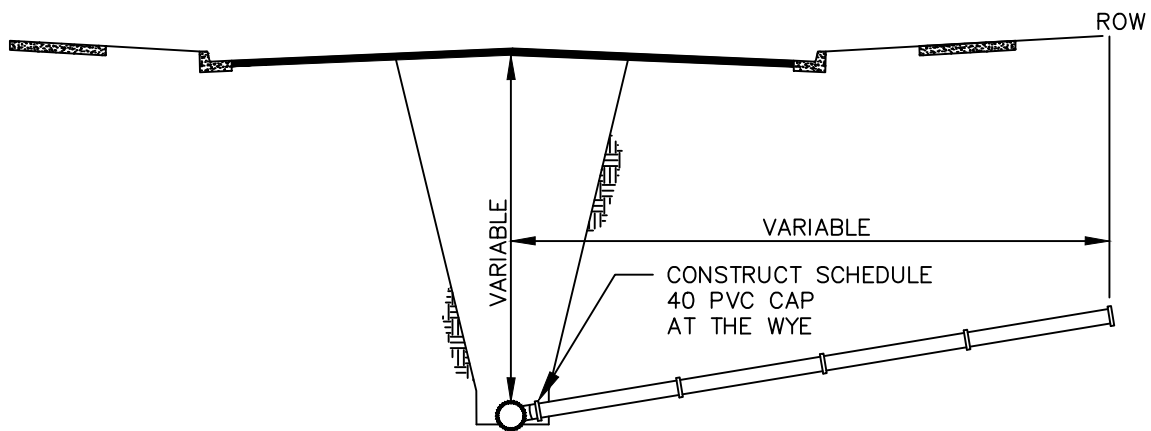
OPTION 1: CAP AT THE WYE
