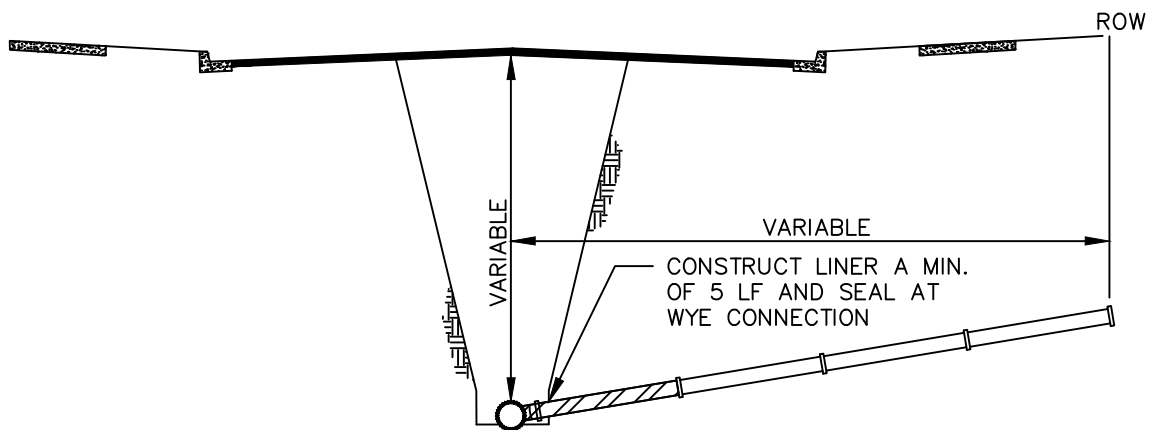
OPTION 2: SERVICE LINER
