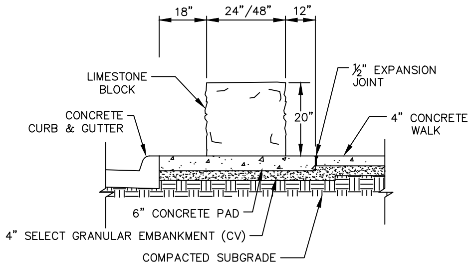
PROFILE VIEW
