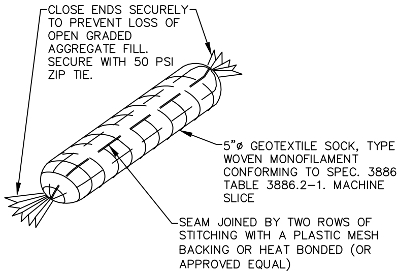
INLET PROTECTION WITH ROCK LOG
