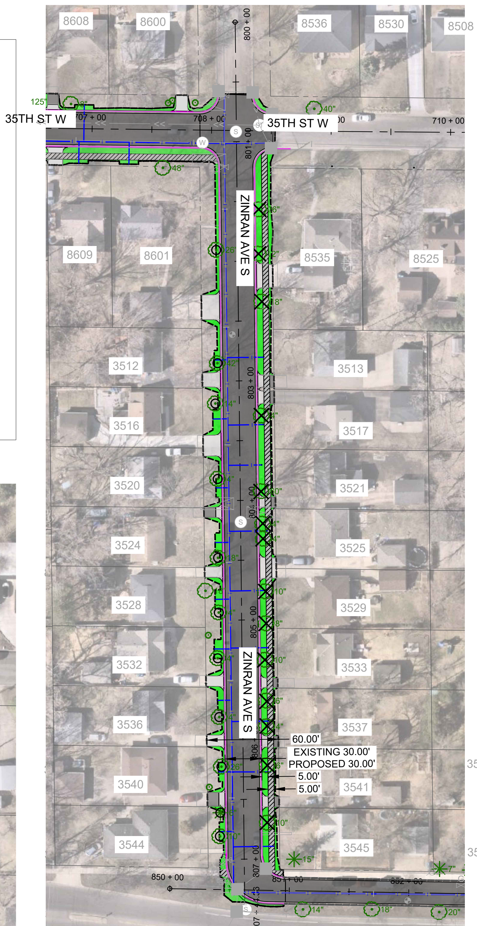
ZINRAN AVE, EAST SIDEWALK OPTION*
